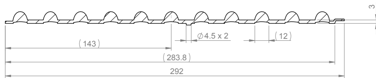
SECTION F-F SCALE 1 : 2
