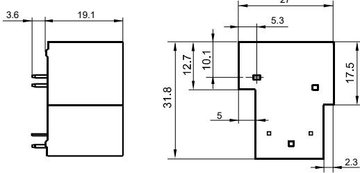
Outline Dimensions
