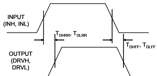
Figure 1—Timing Diagram
