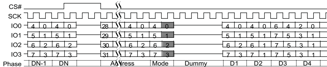
Figure 85. Continuous Quad I/O Read Command Sequence (4-Byte Address), LC=00b
