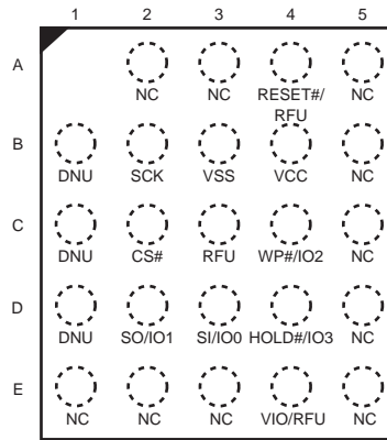
Figure 41. 24-Ball BGA, 5 x 5 Ball Footprint (FAB024), Top View [41]
