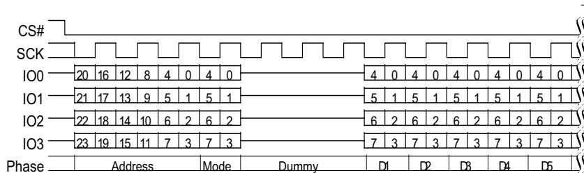
Figure 95. Continuous DDR Quad I/O Read Subsequent Access (3-Byte Address, HPLC=11b)
