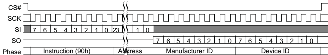
Figure 47. READ_ID (90h) Command Sequence
