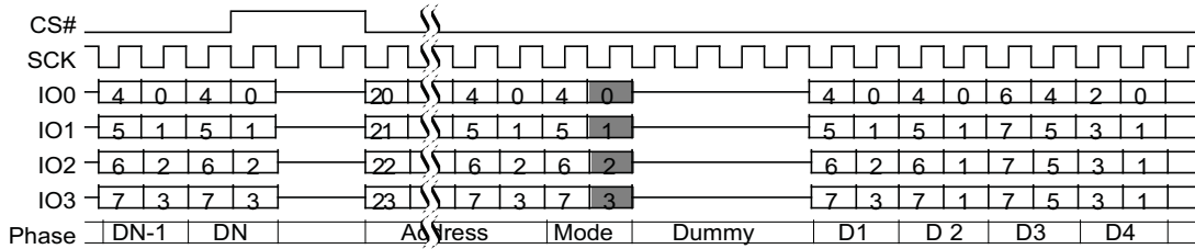
Figure 84. Quad I/O Read Command Sequence(4-Byte Address, ECh or EBh [ExtAdd=1], LC=00b)
