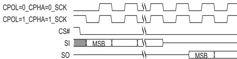
Figure 5. SPI SDR Modes Supported
