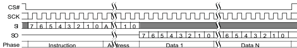
Figure 70. Read Command Sequence (READ 03h or 13h)
