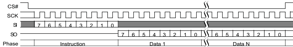
Figure 117. Password Read (PASSRD E7h) Command Sequence
