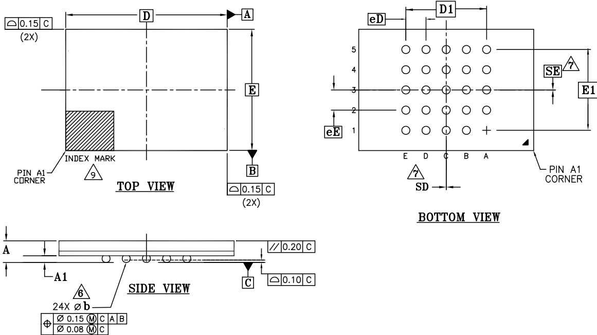
Figure 42. Ball Grid Array 24-Ball 6x8 mm (FAB024)
