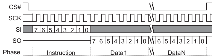
Figure 65. AutoBoot Register Read (ABRD 14h) Command
