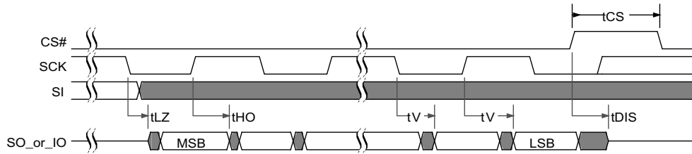
Figure 37. SPI DDR Output Timing
