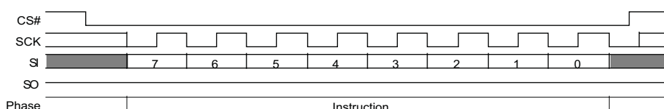
Figure 121. Mode Bit (MBR FFh) Reset Command Sequence
