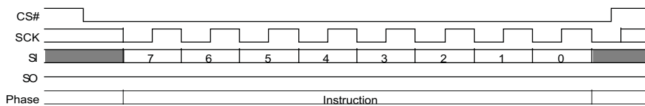
Figure 120. Software Reset (RESET F0h) Command Sequence
