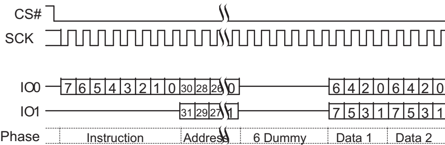
Figure 80. Dual I/O Read Command Sequence (4-Byte Address, BCh or BBh [ExtAdd=1], EHPLC=10b)
