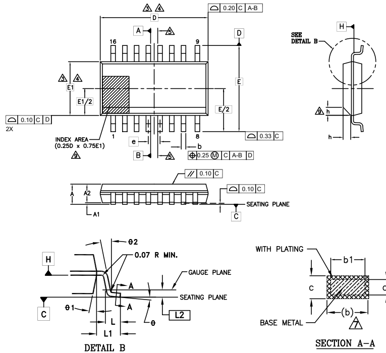
Figure 40. SOIC 16-Lead, 300-mil Body Width (SO3016)
