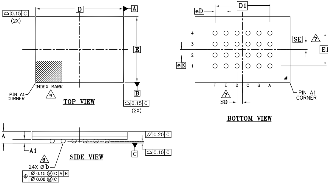
Figure 44. Ball Grid Array 24-Ball 6x8 mm (FAC024)
