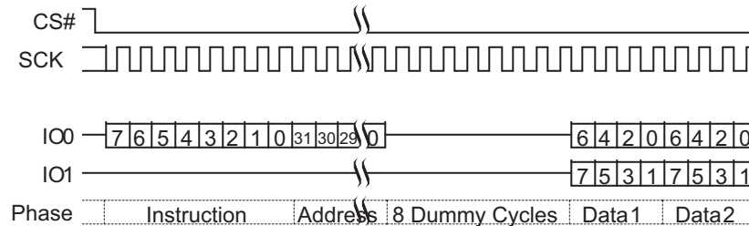
Figure 75. Dual Output Read Command Sequence (4-Byte Address, 3Ch or 3Bh [ExtAdd=1], LC=11b)
