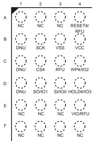
Figure 43. 24-Ball BGA, 4 x 6 Ball Footprint (FAC024), Top View [42]
