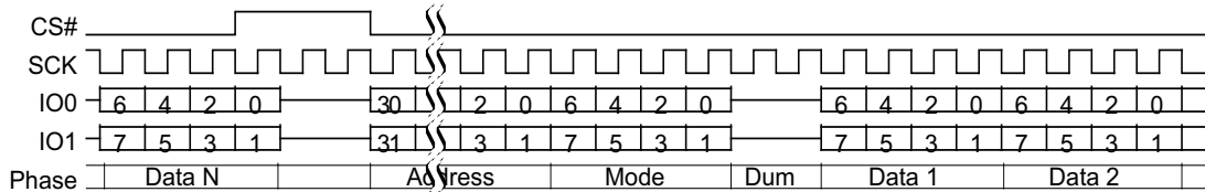
Figure 81. Continuous Dual I/O Read Command Sequence (4-Byte Address, BCh or BBh [ExtAdd=1], EHPLC=10b)
