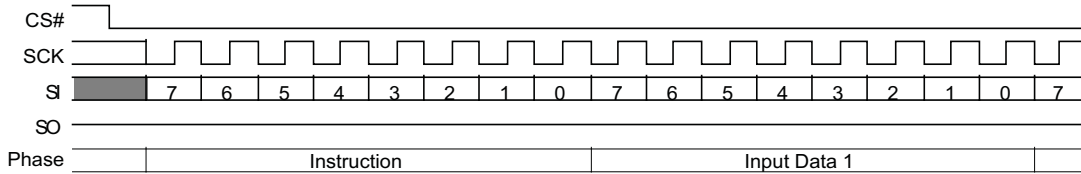
Figure 66. AutoBoot Register Write (ABWR) Command
