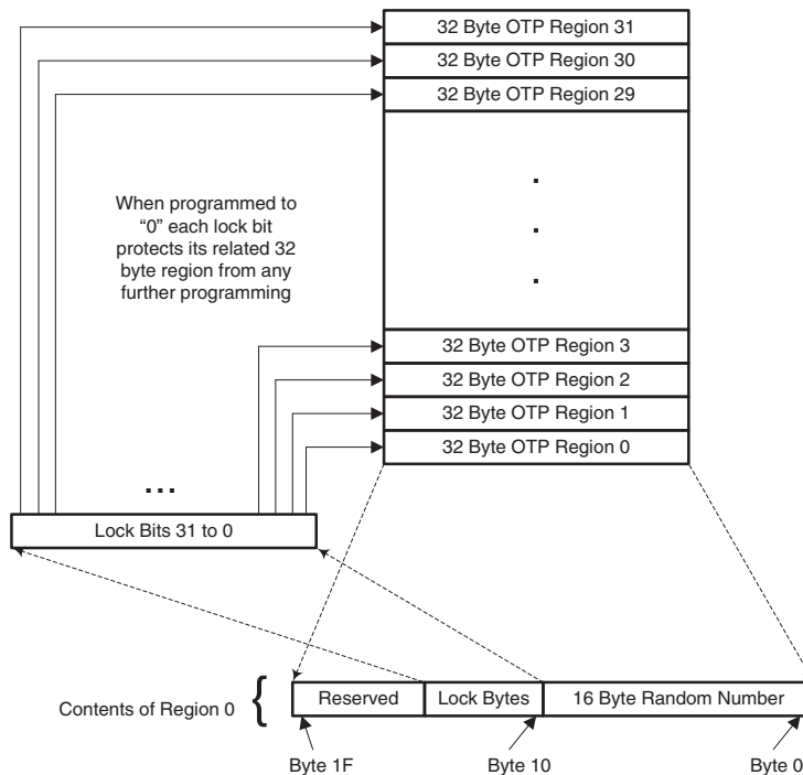
Figure 45. OTP Address Space
