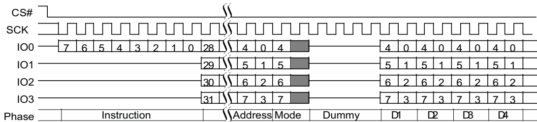
Figure 16. DDR Fast Read with EHPLC = 00b
