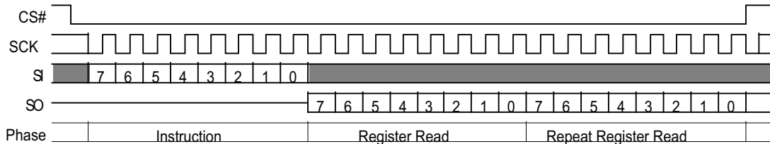
Figure 53. Read Configuration Register (RDCR 35h) Command Sequence
