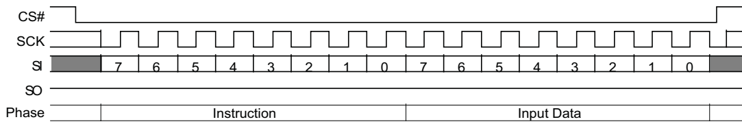
Figure 67. Program NVDLR (PNVDLR 43h) Command Sequence
