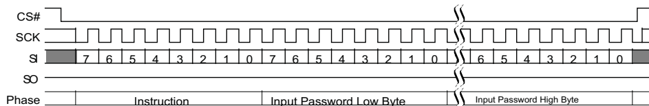
Figure 119. Password Unlock (PASSU E9h) Command Sequence
