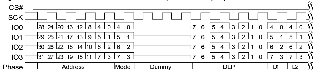
Figure 97. Continuous DDR Quad I/O Read Subsequent Access (4-Byte Address, EHPLC=01b) [48]
