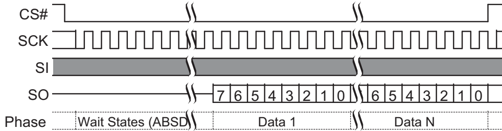
Figure 64. AutoBoot Sequence (CR1[1]=1)
