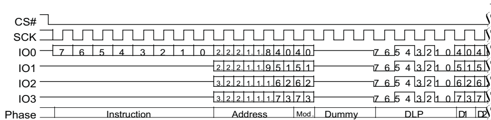
Figure 97. Continuous DDR Quad I/O Read Subsequent Access (4-Byte Address, EHPLC=01b) [48]
