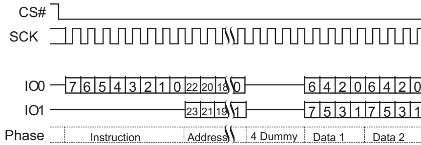
Figure 79. Dual I/O Read Command Sequence (4-Byte Address, BBh [ExtAdd=1], HPLC=10b)
