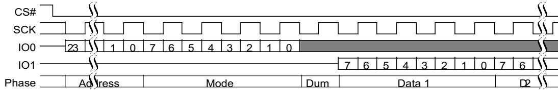
Figure 87. Continuous DDR Fast Read Subsequent Access (3-Byte Address [ExtAdd=0, EHPLC=11b])
