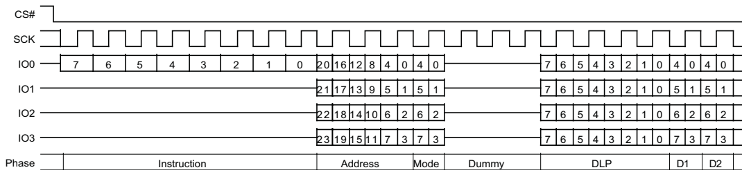
Figure 94. DDR Quad I/O Read Initial Access (3-Byte Address, EDh [ExtAdd=0], HPLC=11b)
