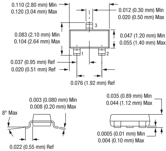
Dimensions are in inches (millimeters shown in parentheses) 200046-009
