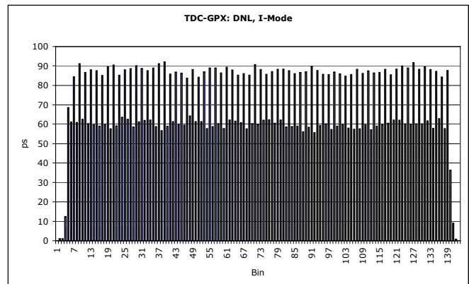
Figure 22: DNL
